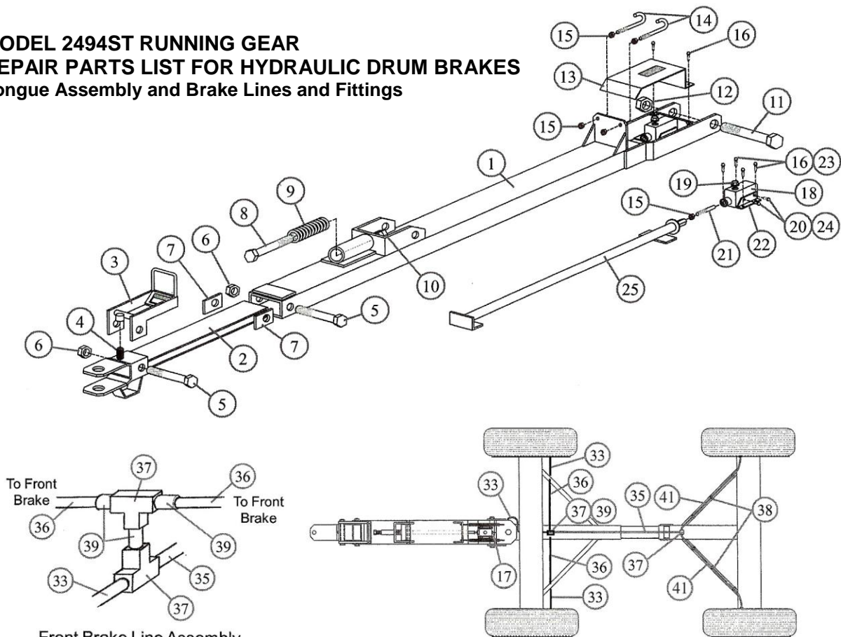
Front Brake Line Assembly PARTS LIST
