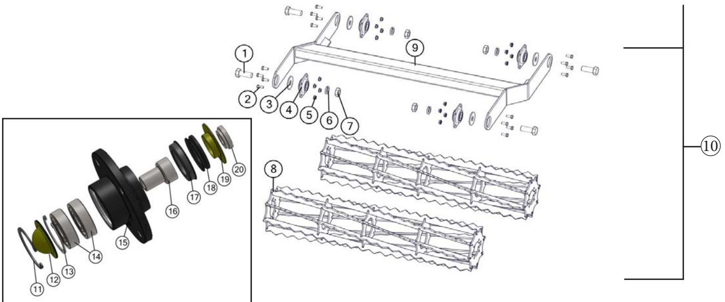
Optional Upgraded Basket Hub
